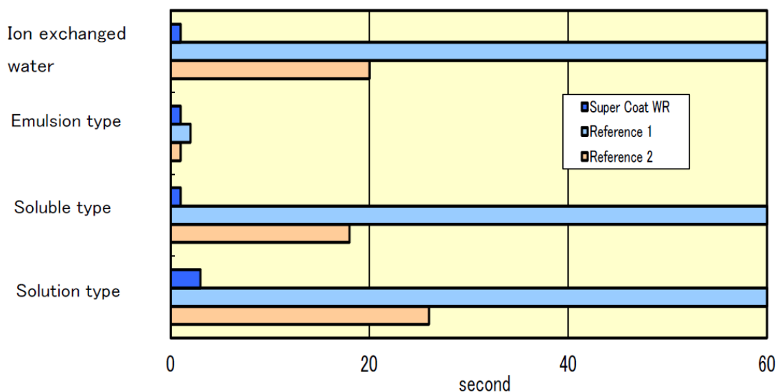
Figure : The time of displacement of ion-exchanged water or water soluble cut oil coated on steel
